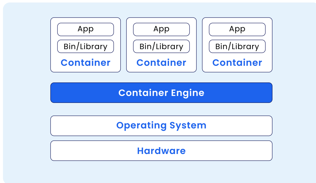
Figure 1: The container engine (or container runtime) is a key component in the container architecture.
